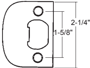
KW-83437 US-3, 5, 10B, 15, 15A Standard Lockset Strike
