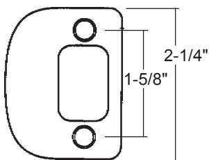
KW-85303 US-10B, 15 Deadbolt strike with lip. 1/4" radius corners.
