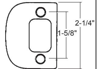
KW-84638 US-3, 26D Deadbolt strike with lip
