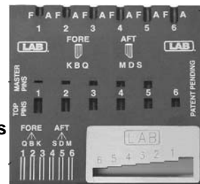
LB-LFT 005 Set of Five Followers Below LB-LFT 000 Schlage (For 3 types of cylinders) LB-LFT 001 Universal (.498) LFT 002 Weslock (.500) Dia. LFT 003 Corbin (.550) Dia. LFT 004 Small Plug (.398) Dia. • Light weight • Very Durable • White Delrin* • Reflects Light for pinning *Delrin is a product of Dupont Industries
