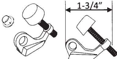
CR-DSLD81 US-3, 5, 10B, 15, 26D Residential (light duty) Hinge Pin Stop w/nylon bushing.
