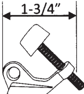
CR-DSLD81 US-3, 5, 10B, 15, 26D Residential (light duty) Hinge Pin Stop w/nylon bushing.
