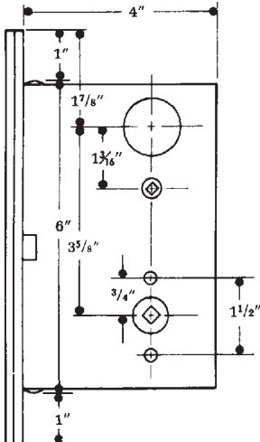
GLOBAL (GWM) knob with escutcheon
